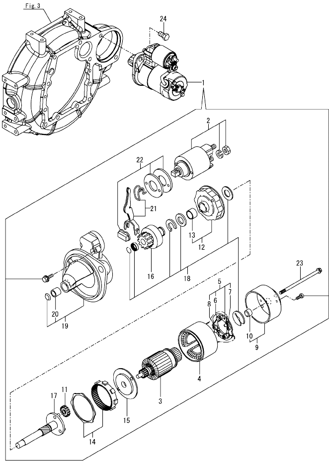
Fig.15. STARTER MOTOR
