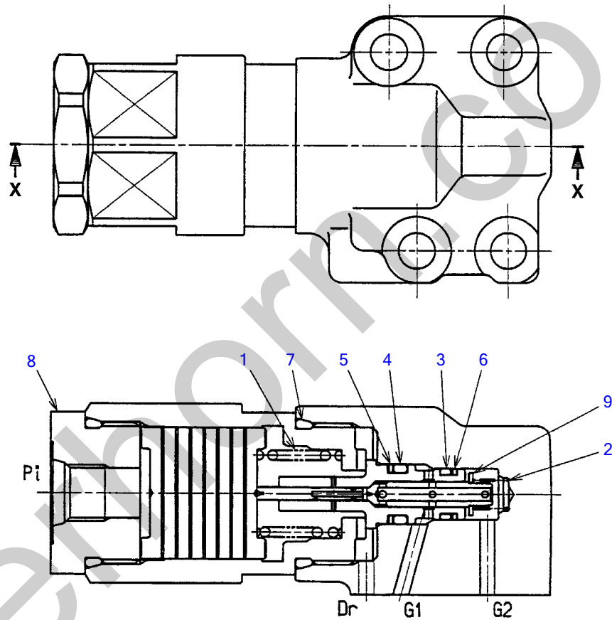
SECTION "X-X"
